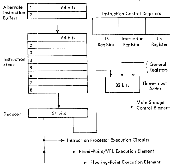
Figure 5. Instruction Processor
